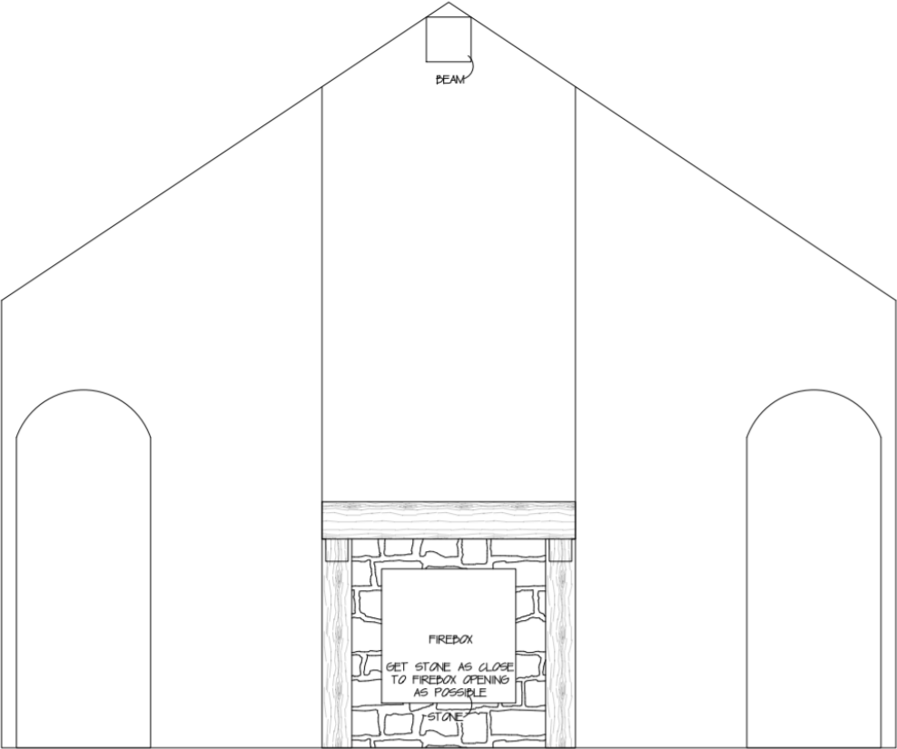
FIREPLACE WALL ELEVATION
