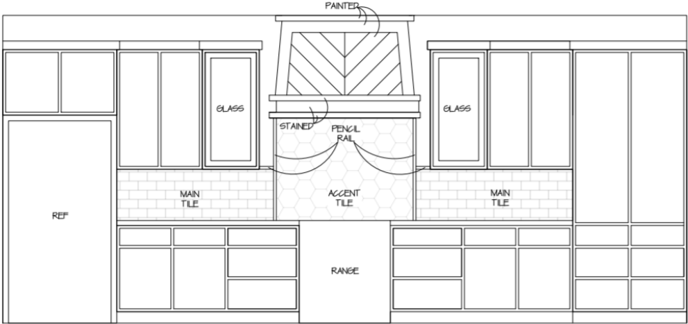
KITCHEN CABINET ELEVATIONS SHAKER STYLE CABINET DOORS
