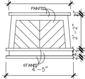
VENT HOOD DETAILS 4'-0 1/2"
