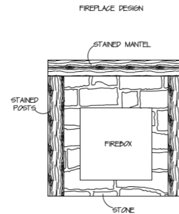
FIREPLACE ELEVATION
